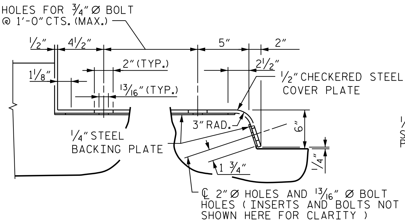
DETAIL "B"
