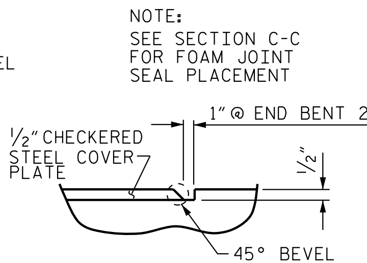
DETAIL "C"
