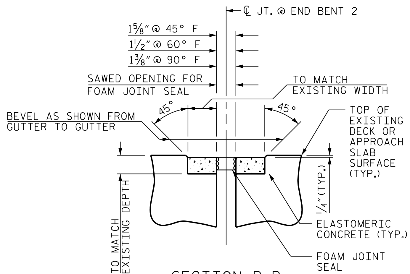
SECTION B-B
