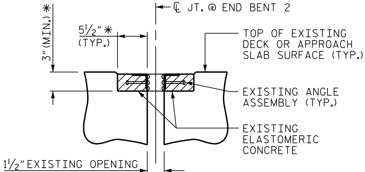
SECTION B-B
